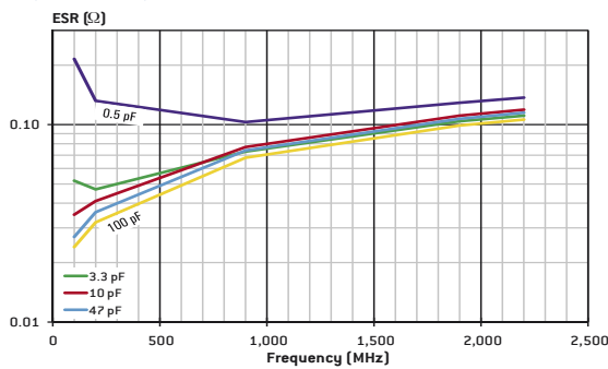
SHF (SIZE 0805): TYPICAL ESR VERSUS FREQUENCY
