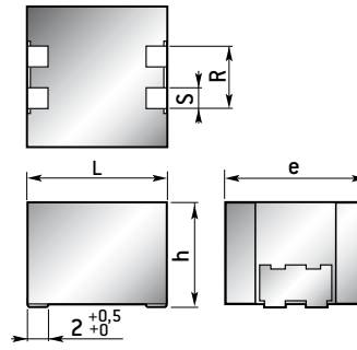
SMD leads Model KM 94 - KM 94 S
